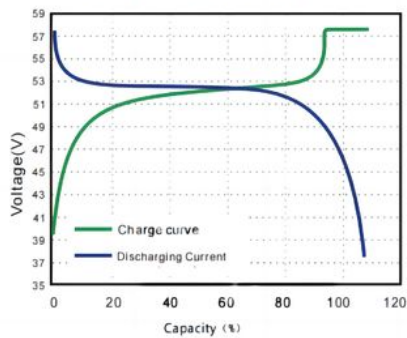
● Charge and discharge curve @0.5C 25°C
