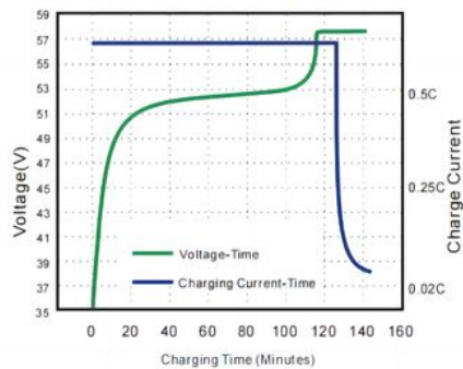
● Charging Characteristics @0.5C 25°C
